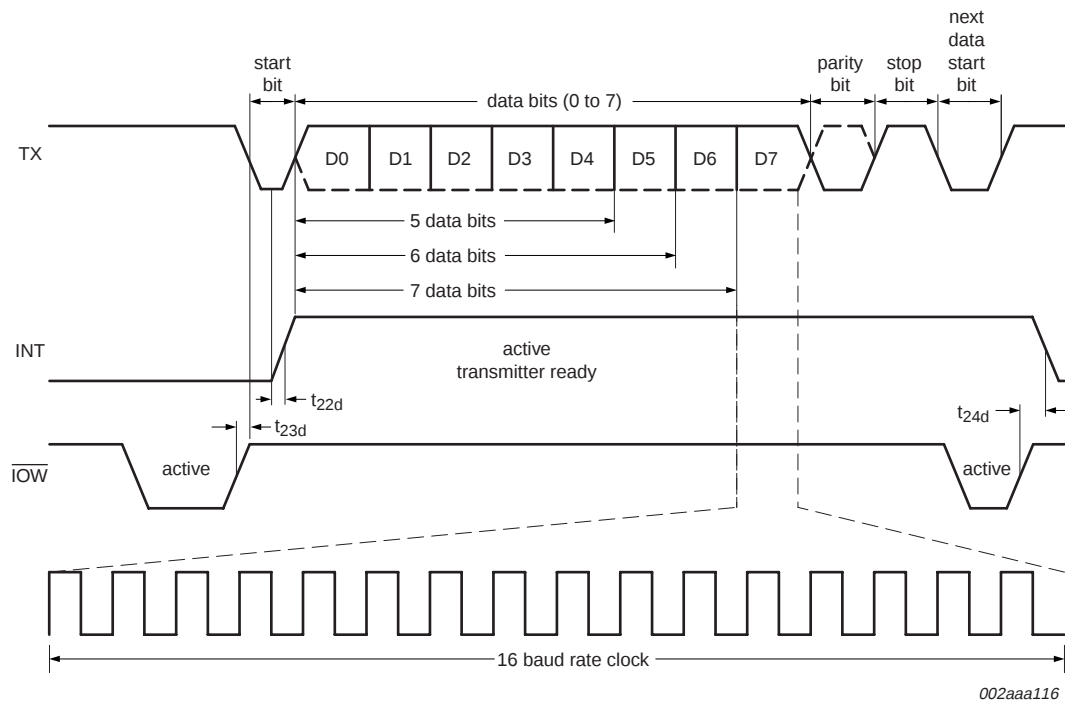
Fig 18. Transmit timing.
