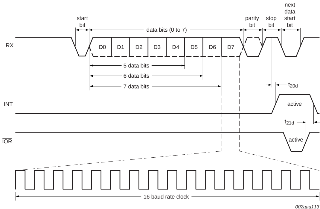
Fig 15. Receive timing.
